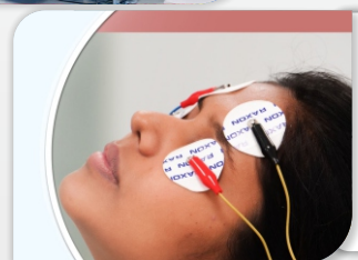
Micro Currents
